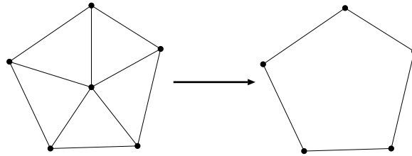
図 7.8: removeVertexInLoop
