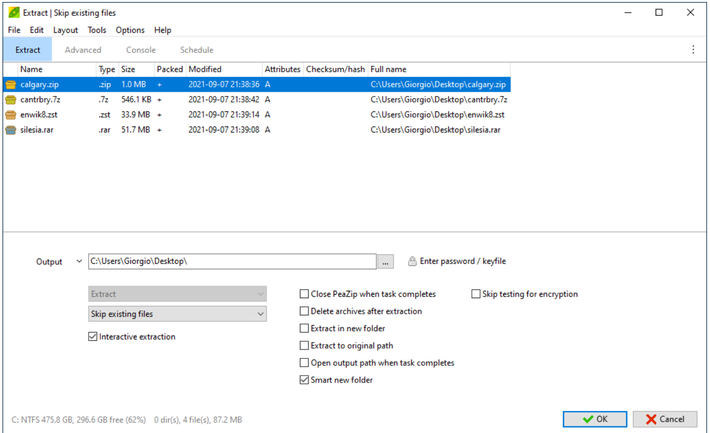
Image 15: Extraction interface: rightclick the input area, or click the menu icon on the top right of the application, to display the context menu to add/remove objects from extraction layout, and display other related functions.
