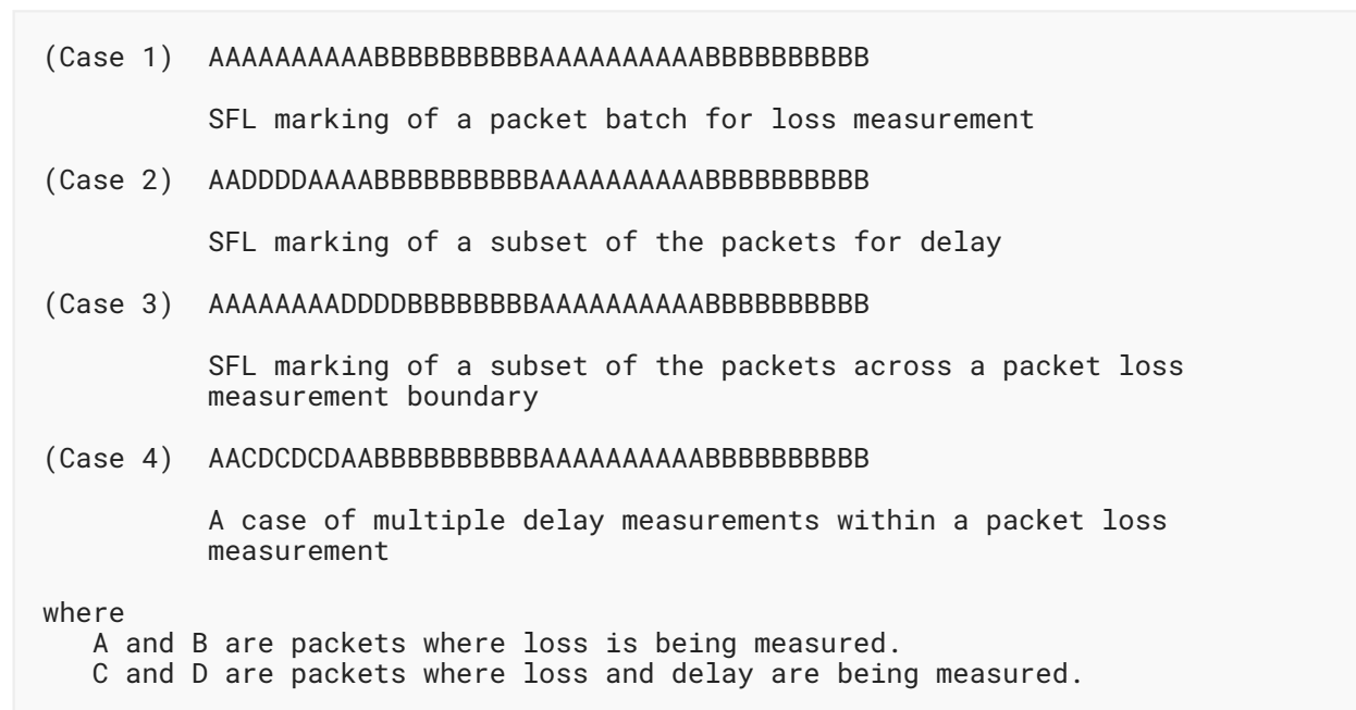
Figure 1: RFC 6734 Query Packet with SFL
